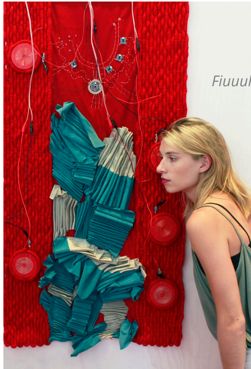
Sound Space Shell with capacitive sensor area and stiched textile speakers.
