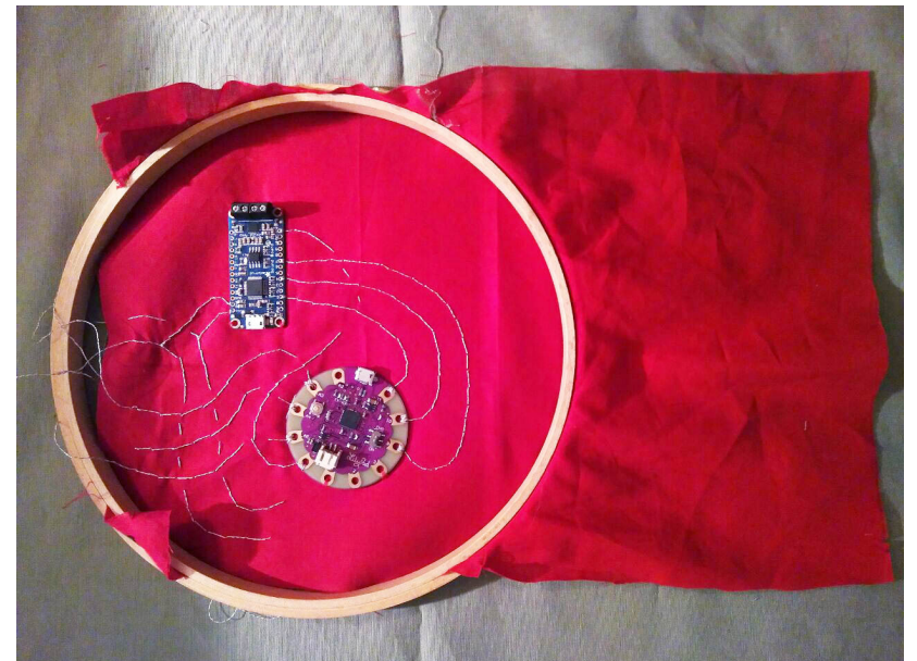
Sewing a textile circuit with conductive yarn, soundboard and microcontroller.
